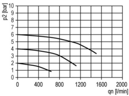
flow characteristic
